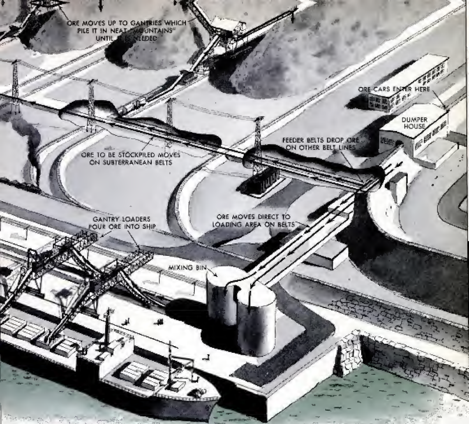
Artist's drawing shows ore terminal at Seven Islands. Ore moves on subterranean belts to ship or stock piles. Right, map shows location of ore zone and railroad
